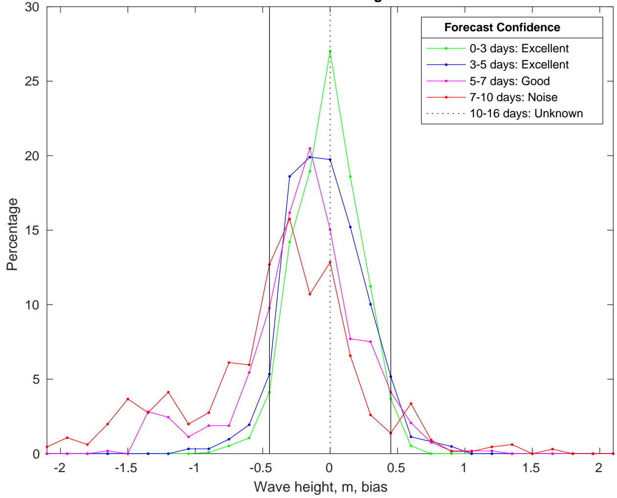
NDBC 42084 vs CMEMSWaves Bias Histogram: 17-Jan-2025
