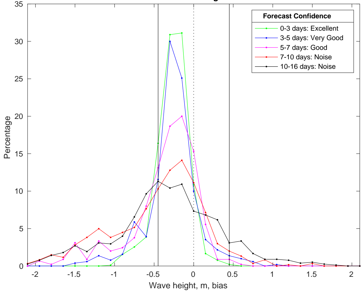
NDBC 42084 vs GFSWaves Bias Histogram: 17-Jan-2025
