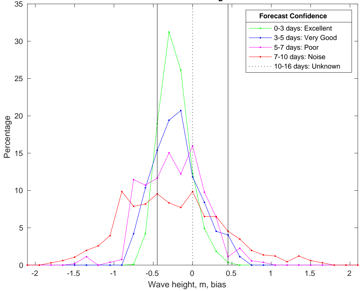
NDBC 42092 vs CMEMSWaves Bias Histogram: 17-Jan-2025
