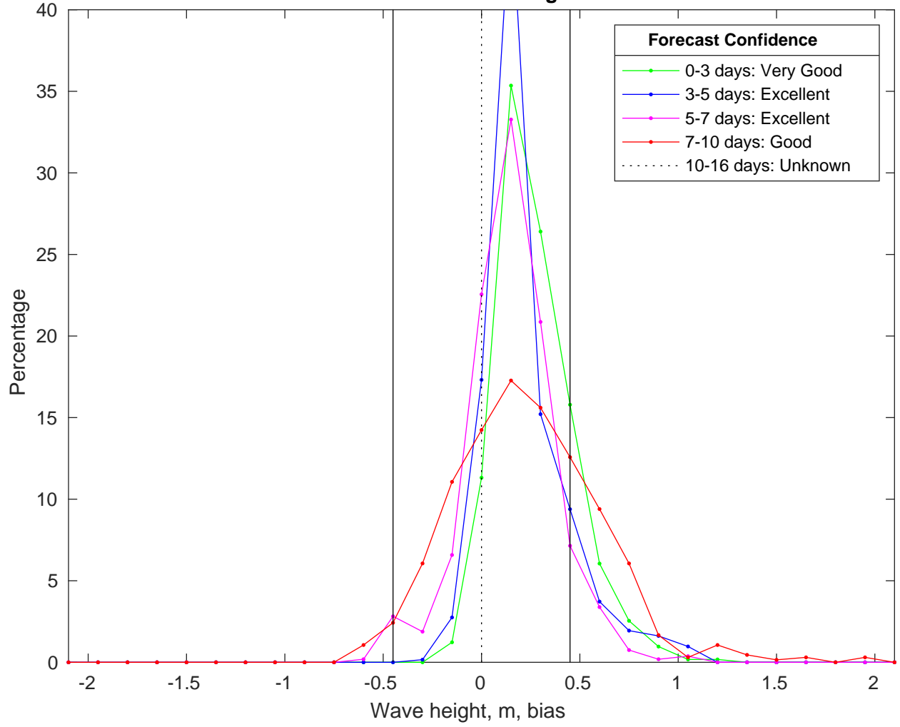
NDBC 44020 vs CMEMSWaves Bias Histogram: 17-Jan-2025
