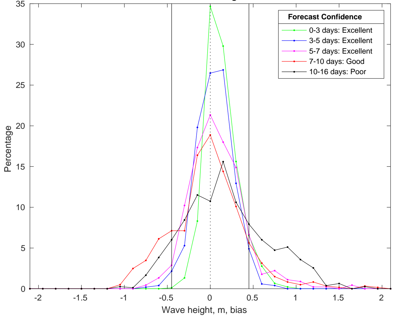
NDBC 44020 vs GFSWaves Bias Histogram: 17-Jan-2025
