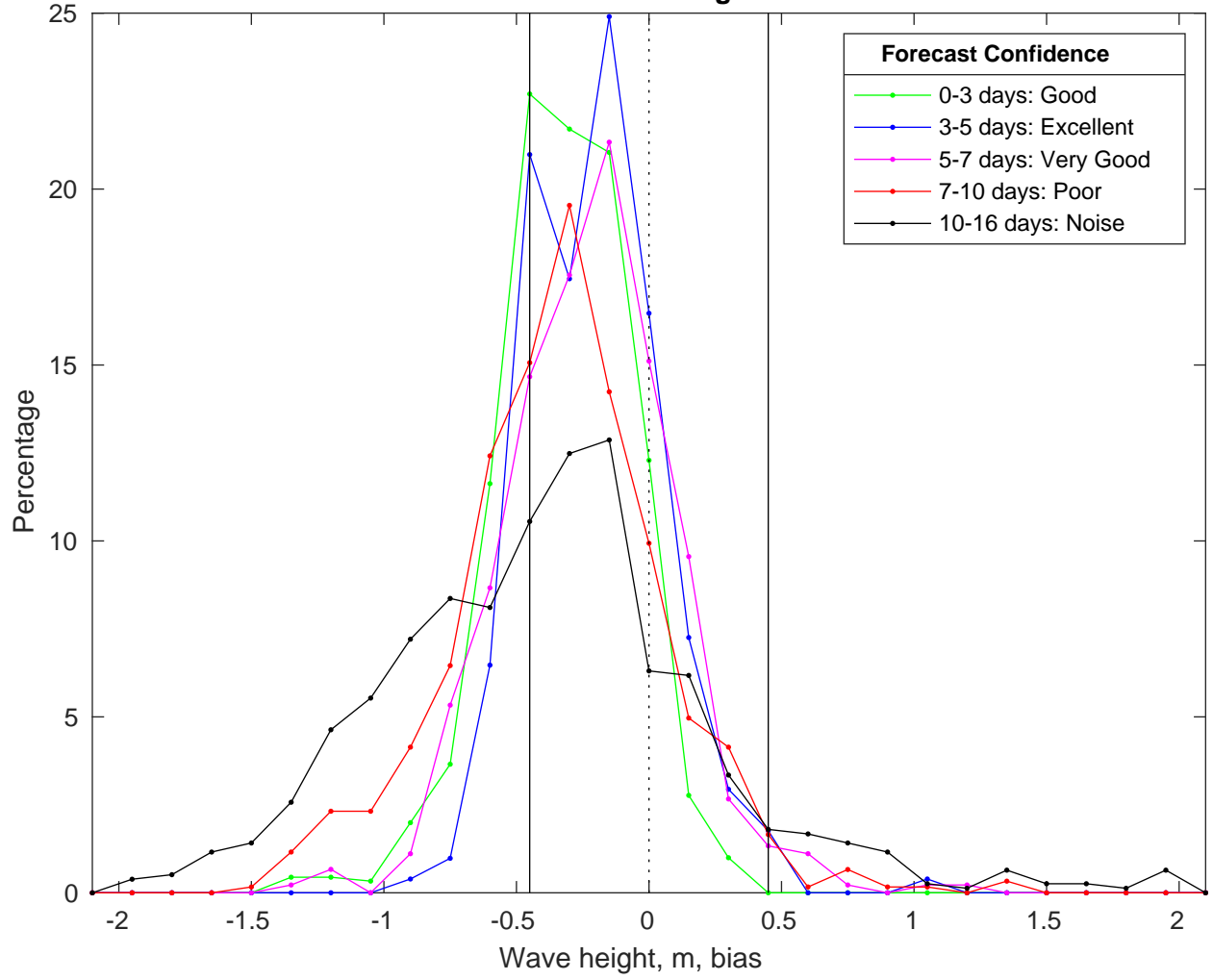
NDBC 46011 vs GFSWaves Bias Histogram: 17-Jan-2025
