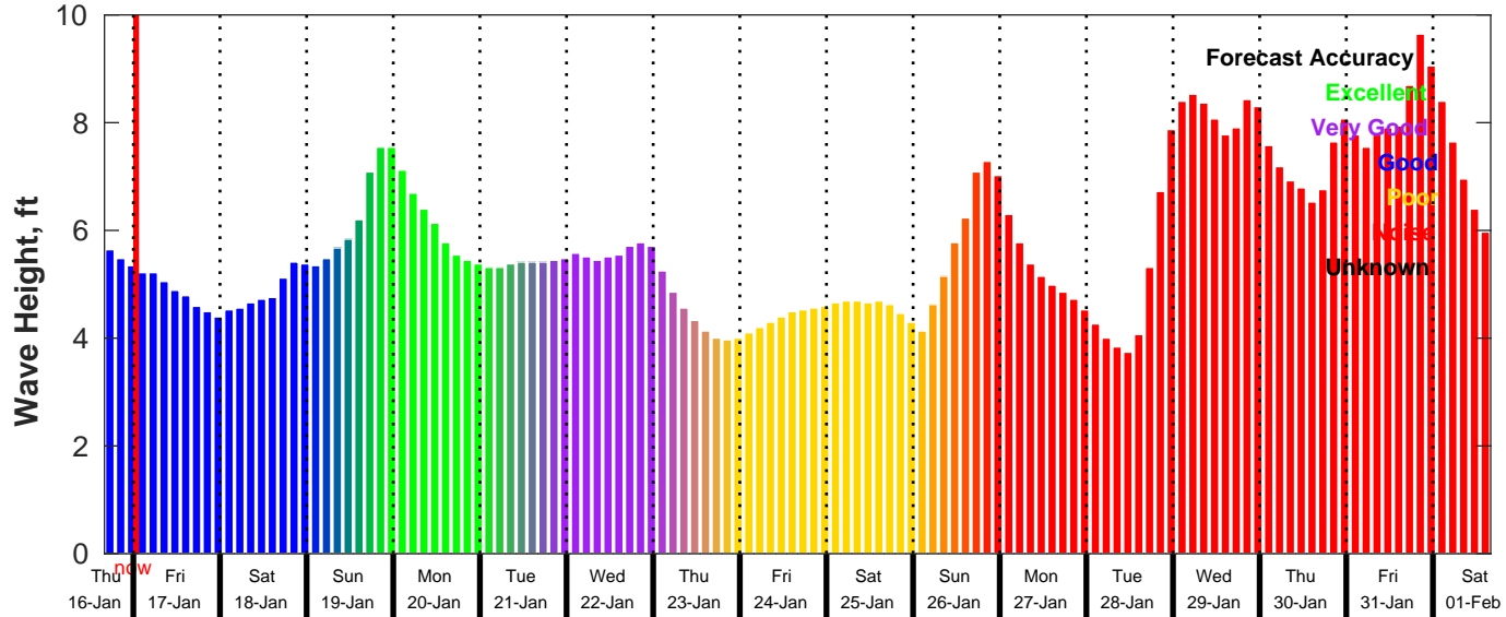
GFS Wave Forecast for NDBC 46011 from 16-Jan-2025 16:00:00 to 01-Feb-2025 16:00:00
