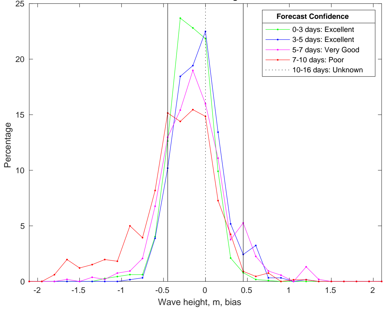
NDBC 46028 vs CMEMSWaves Bias Histogram: 17-Jan-2025
