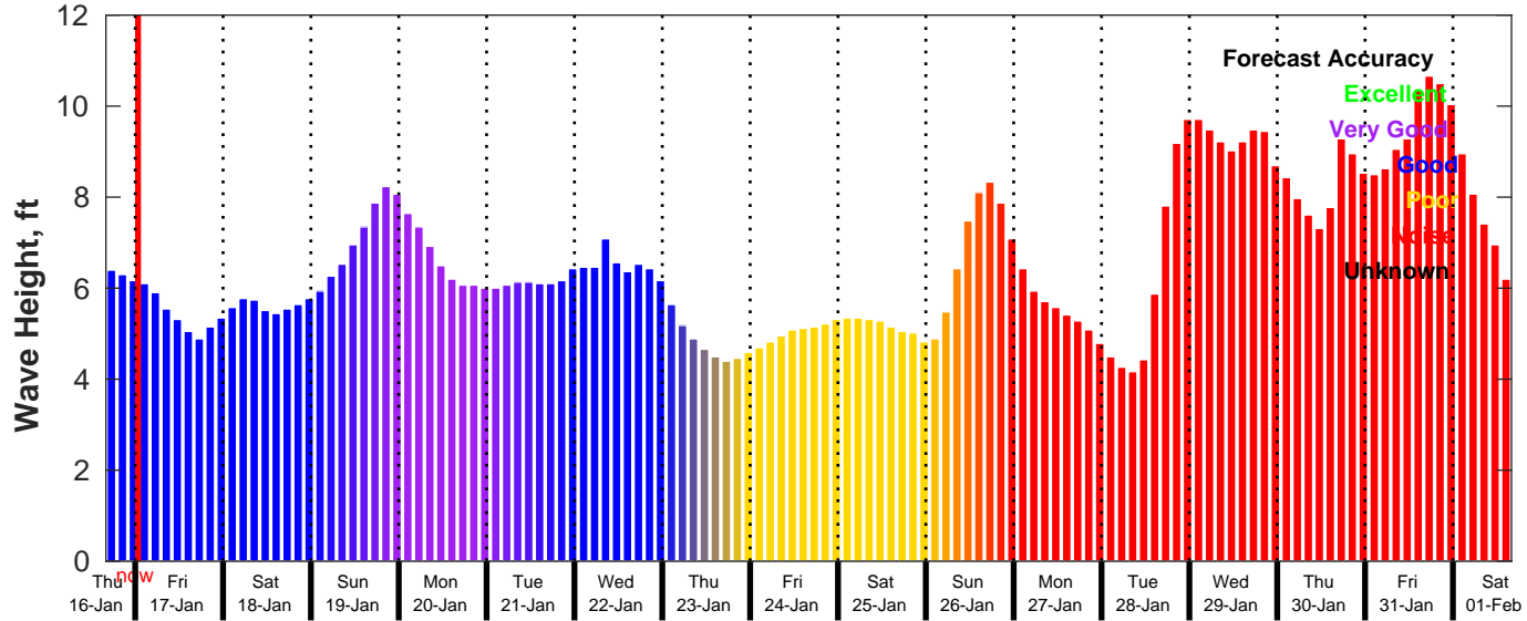
GFS Wave Forecast for NDBC 46028 from 16-Jan-2025 16:00:00 to 01-Feb-2025 16:00:00
