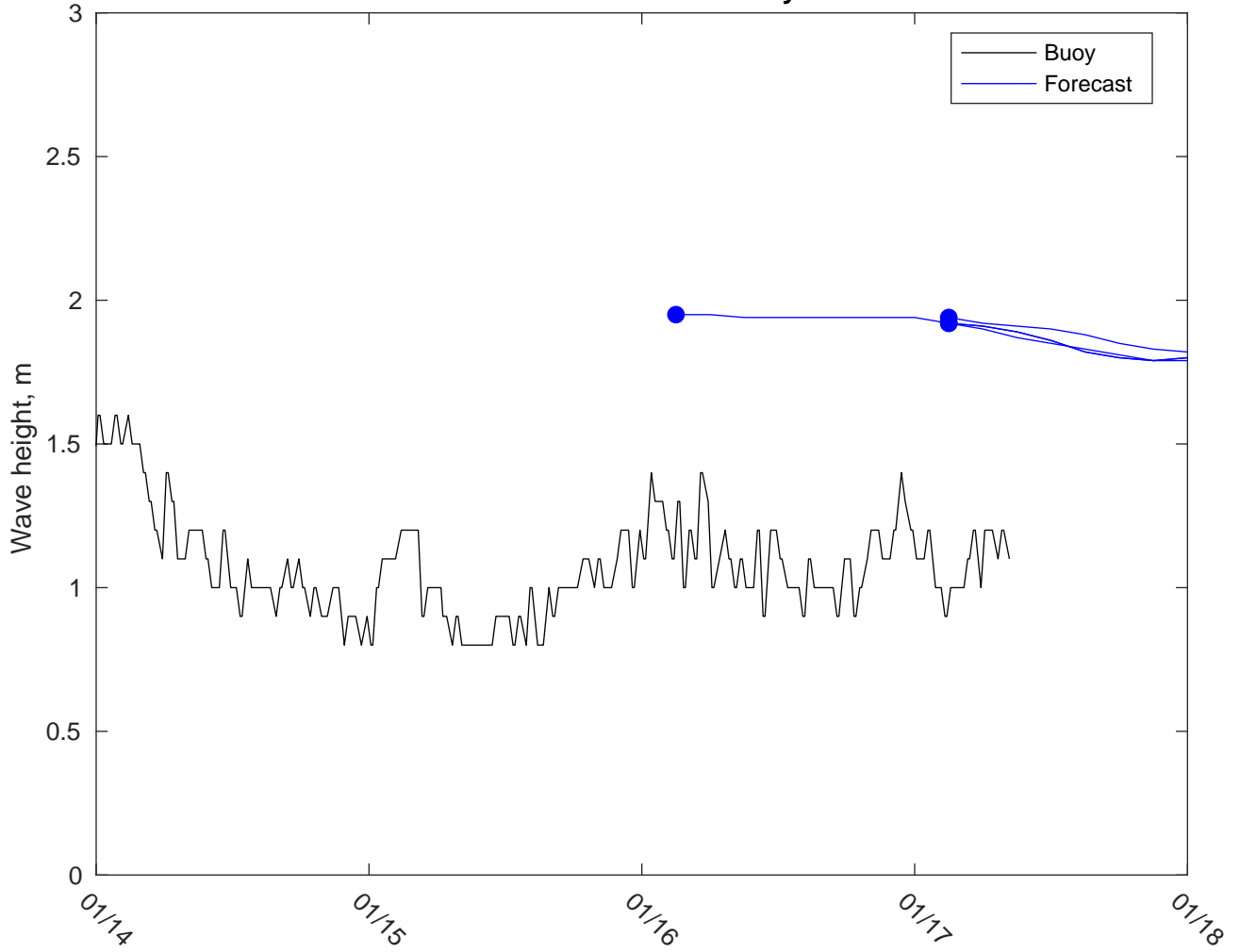
NDBC 46053 vs CMEMSWaves: 3 to 5 day forecast
