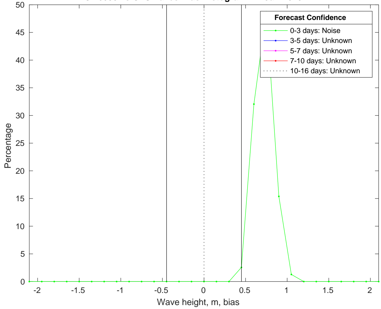
NDBC 46053 vs GFSWaves Bias Histogram: 17-Jan-2025
