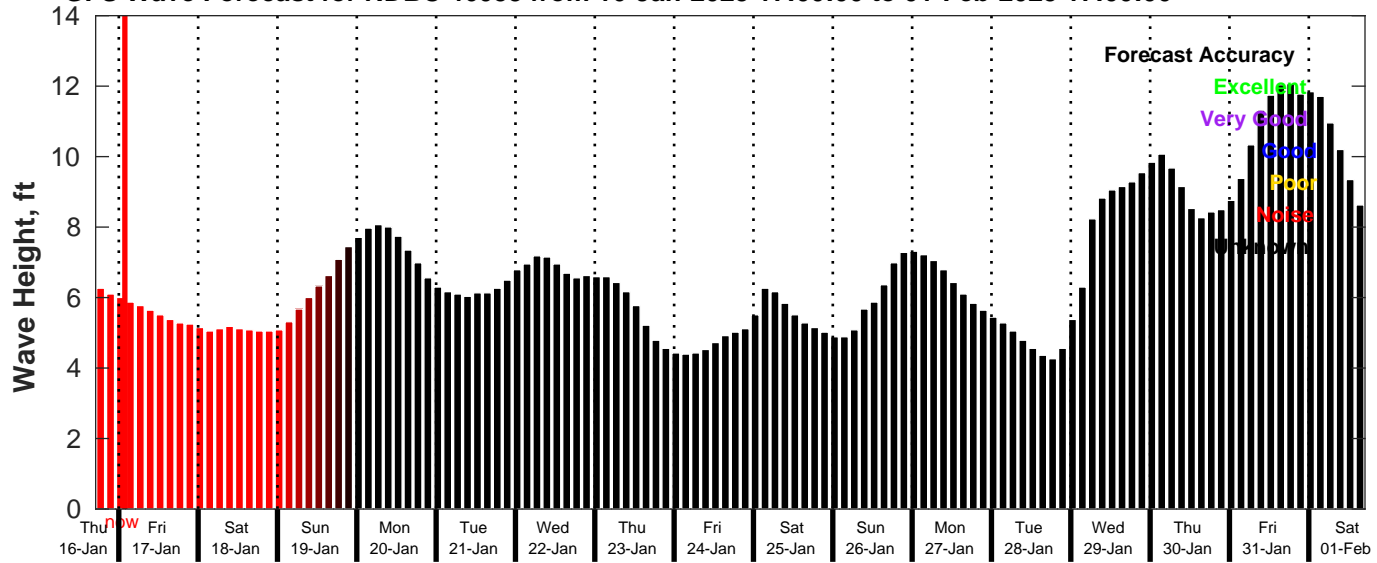
GFS Wave Forecast for NDBC 46053 from 16-Jan-2025 17:00:00 to 01-Feb-2025 17:00:00
