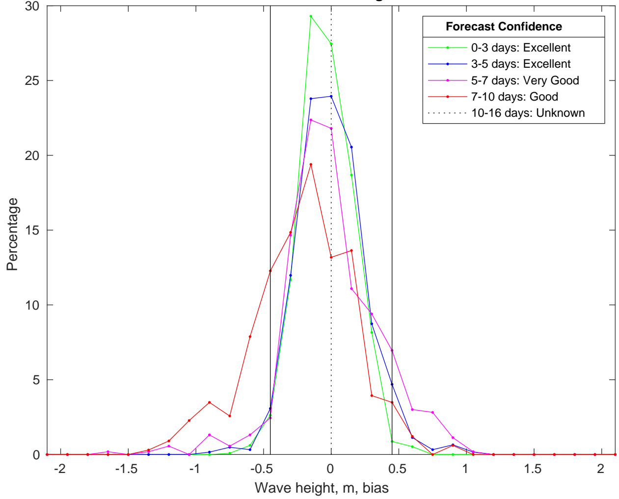
NDBC 46054 vs CMEMSWaves Bias Histogram: 17-Jan-2025
