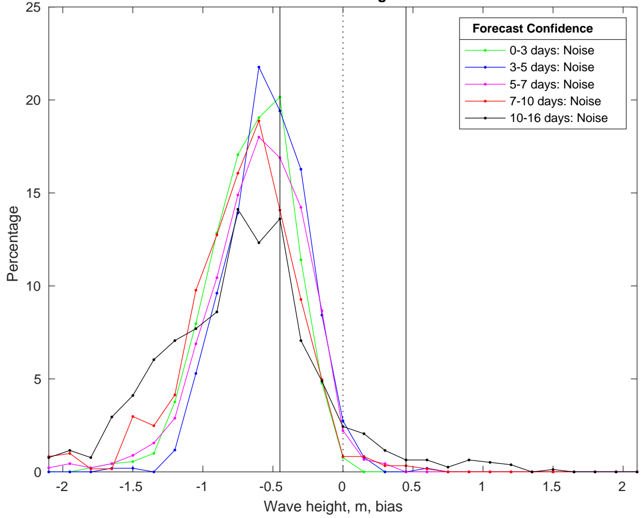
NDBC 46054 vs GFSWaves Bias Histogram: 17-Jan-2025
