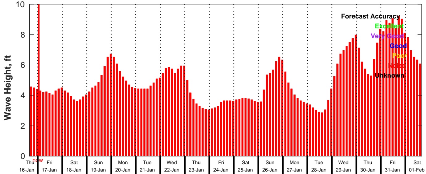
GFS Wave Forecast for NDBC 46069 from 16-Jan-2025 16:00:00 to 01-Feb-2025 16:00:00
