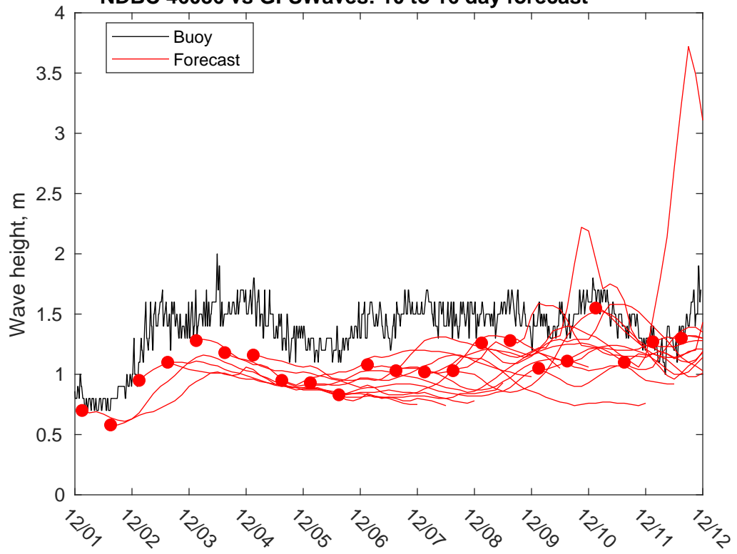
NDBC 46086 vs GFSWaves: 10 to 16 day forecast
