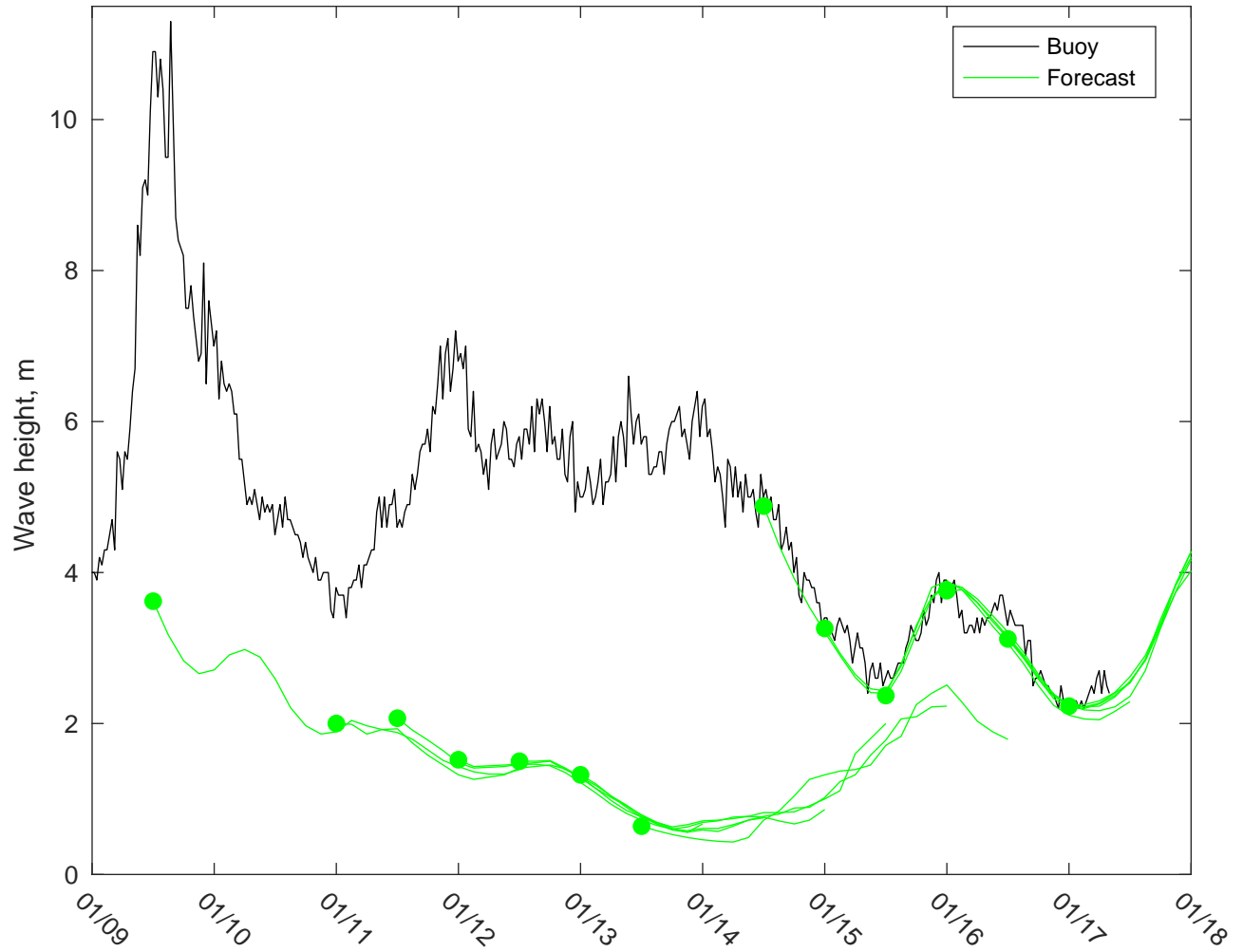
NDBC 46246 vs GFSWaves: 0 to 3 day forecast
