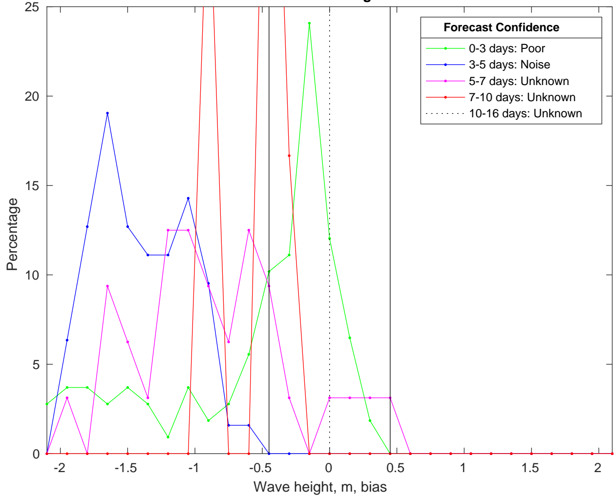
NDBC 46246 vs GFSWaves Bias Histogram: 17-Jan-2025
