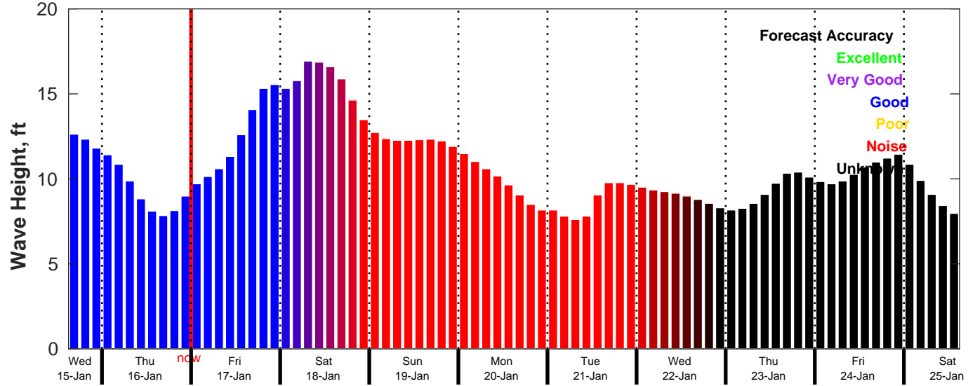
CMEMS Wave Forecast for NDBC 46246 from 15-Jan-2025 15:00:00 to 25-Jan-2025 15:00:00
