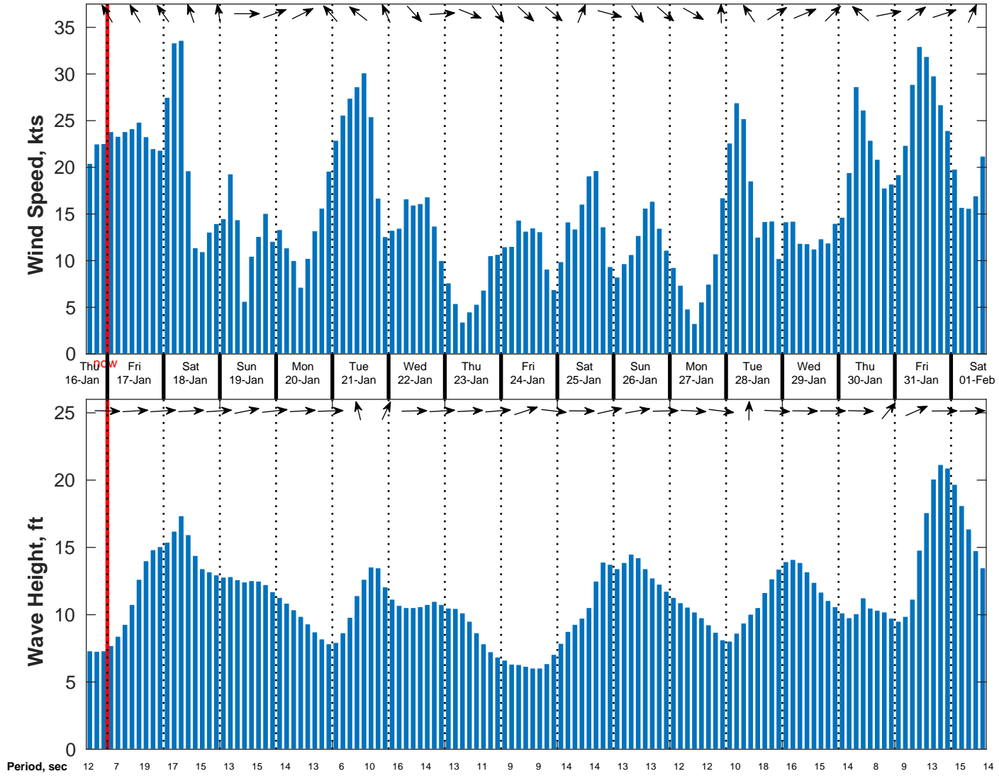
Wind & Wave Forecast for NDBC 46246 from 16-Jan-2025 15:00:00 to 01-Feb-2025 15:00:00
