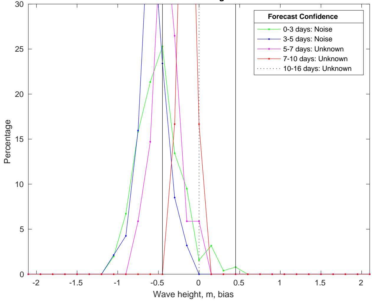
NDBC 51209 vs GFSWaves Bias Histogram: 17-Jan-2025
