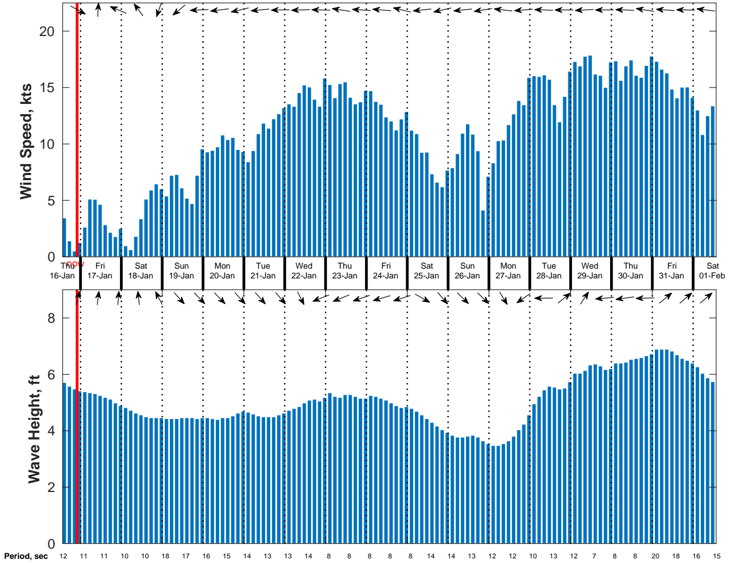
Wind & Wave Forecast for NDBC 51209 from 16-Jan-2025 13:00:00 to 01-Feb-2025 13:00:00
