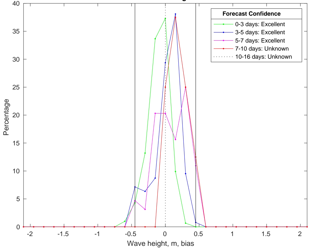
NDBC 52211 vs GFSWaves Bias Histogram: 17-Jan-2025
