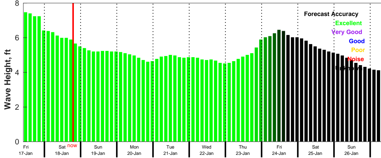
CMEMS Wave Forecast for NDBC 52211 from 16-Jan-2025 10:00:00 to 26-Jan-2025 10:00:00
