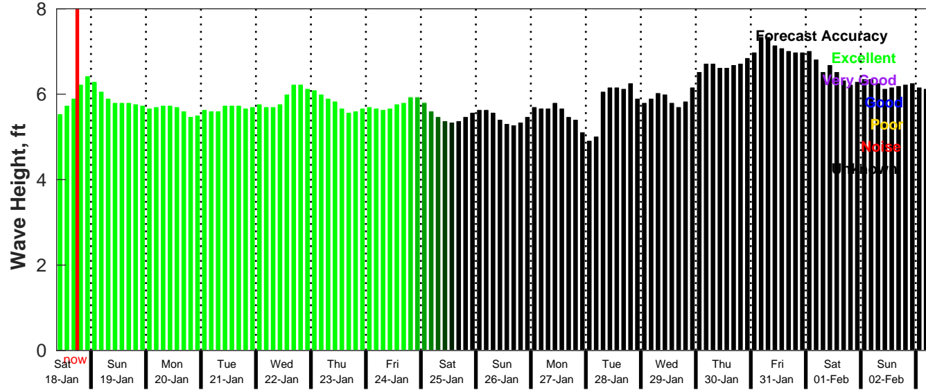
GFS Wave Forecast for NDBC 52212 from 17-Jan-2025 09:00:00 to 02-Feb-2025 09:00:00
