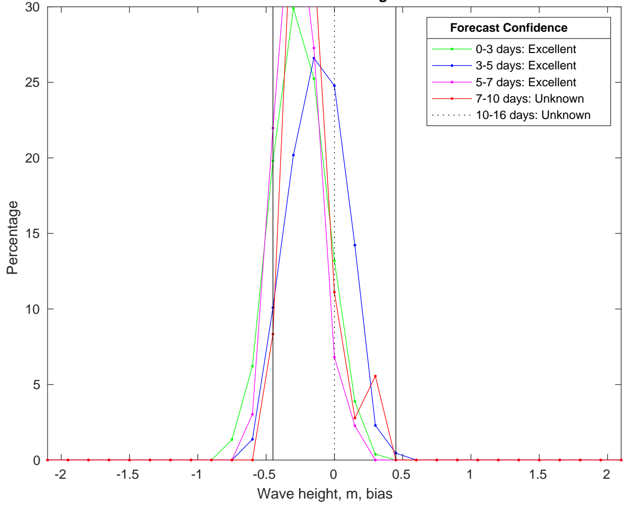
NDBC 52213 vs CMEMSWaves Bias Histogram: 17-Jan-2025
