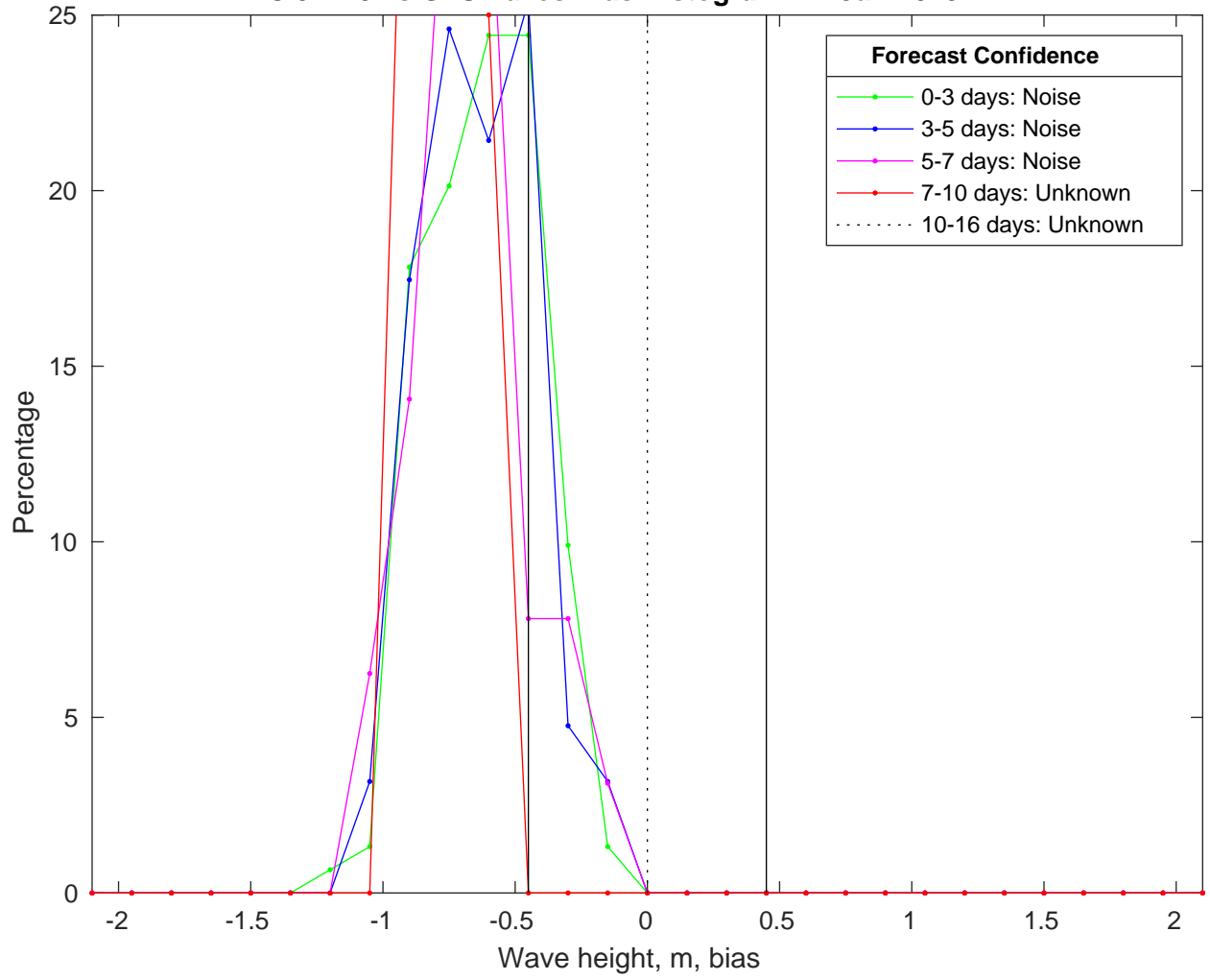
NDBC 52213 vs GFSWaves Bias Histogram: 17-Jan-2025
