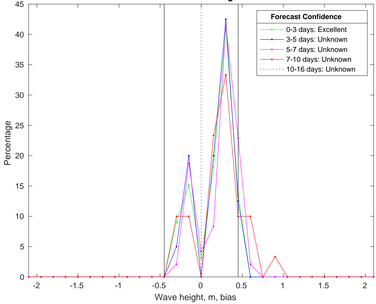
NDBC 62305 vs CMEMSWaves Bias Histogram: 17-Jan-2025
