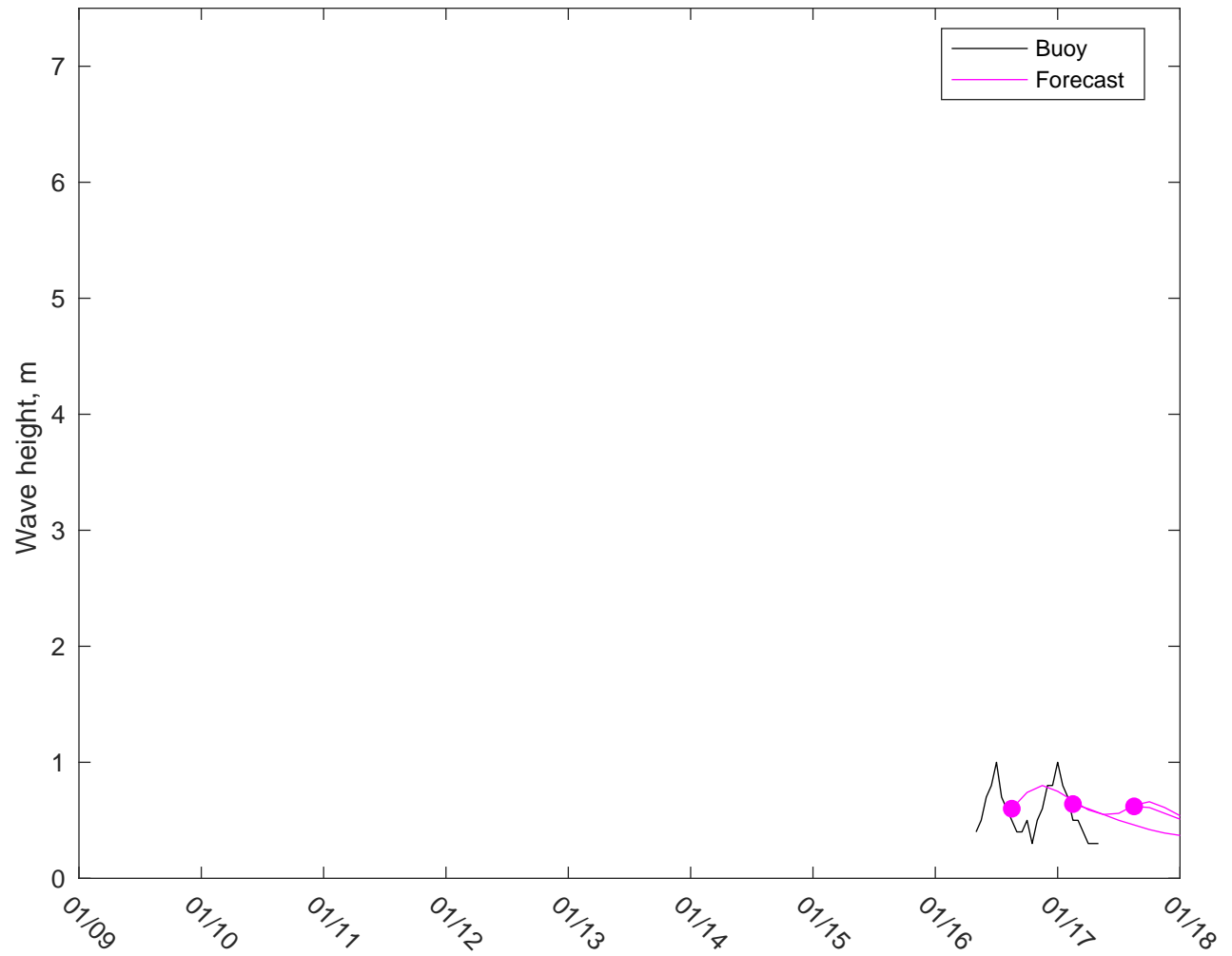
NDBC 62305 vs GFSWaves: 7 to 10 day forecast
