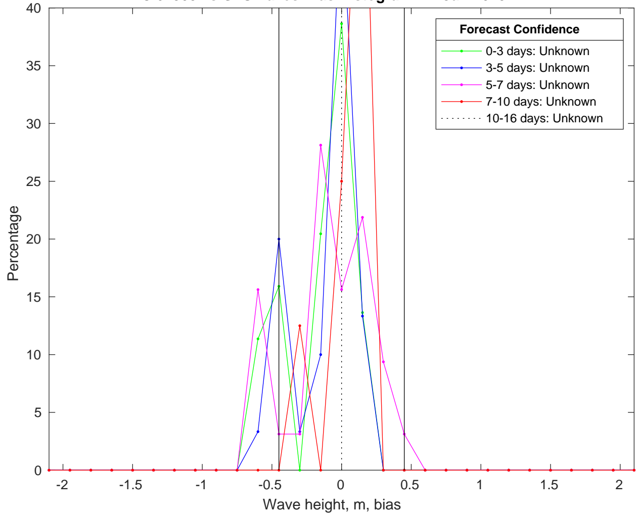
NDBC 62305 vs GFSWaves Bias Histogram: 17-Jan-2025
