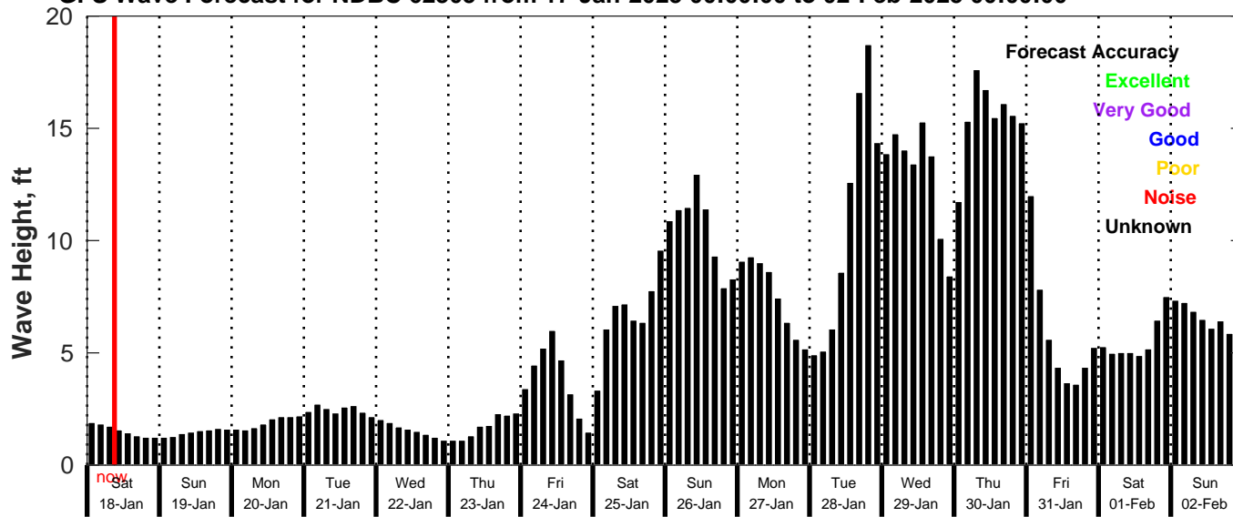
GFS Wave Forecast for NDBC 62305 from 17-Jan-2025 00:00:00 to 02-Feb-2025 00:00:00
