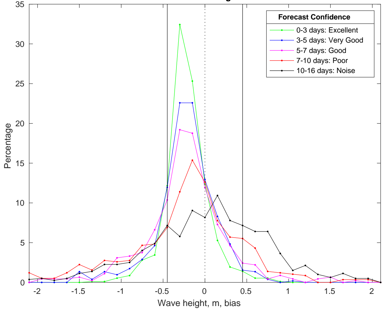
NDBC 41004 vs GFSWaves Bias Histogram: 18-Jan-2025
