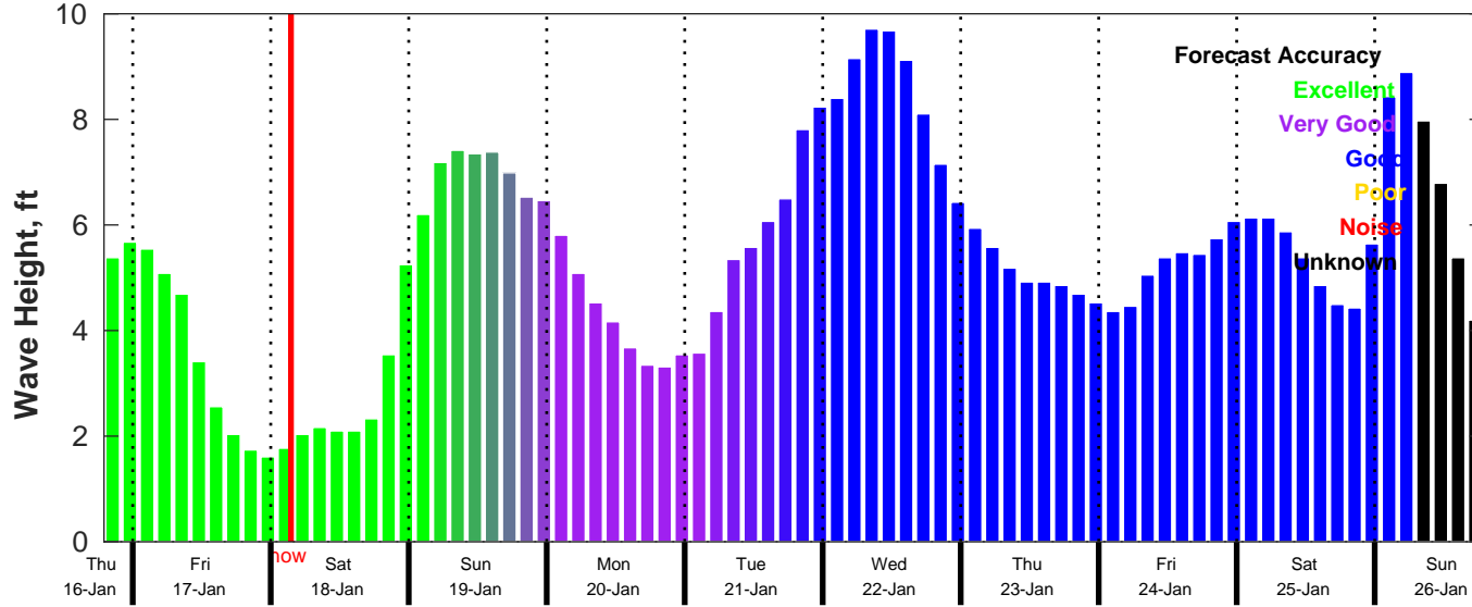
CMEMS Wave Forecast for NDBC 41004 from 16-Jan-2025 19:00:00 to 26-Jan-2025 19:00:00
