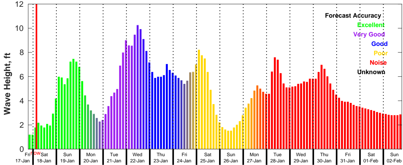
GFS Wave Forecast for NDBC 41004 from 17-Jan-2025 19:00:00 to 02-Feb-2025 19:00:00
