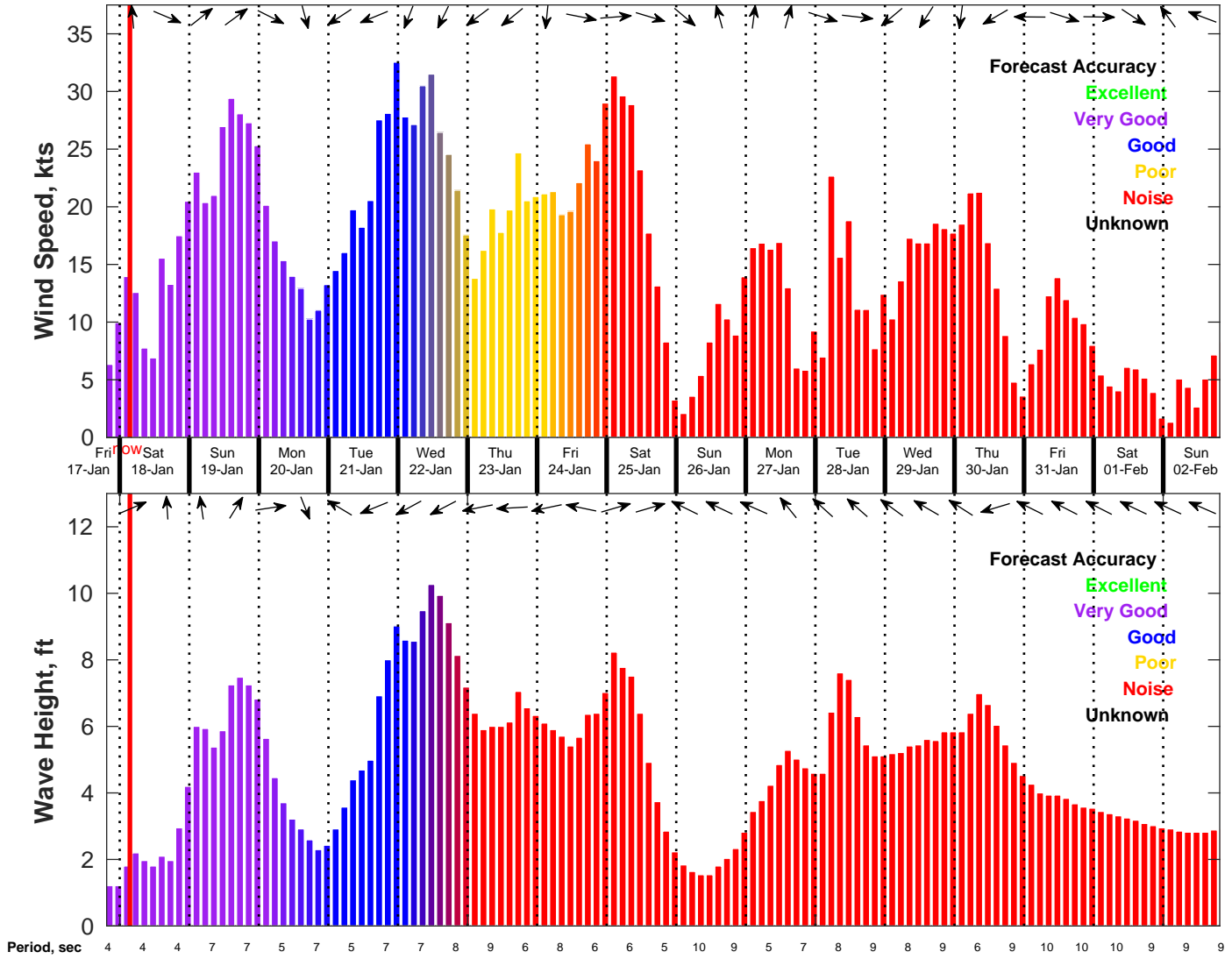
Wind & Wave Forecast for NDBC 41004 from 17-Jan-2025 19:00:00 to 02-Feb-2025 19:00:00
