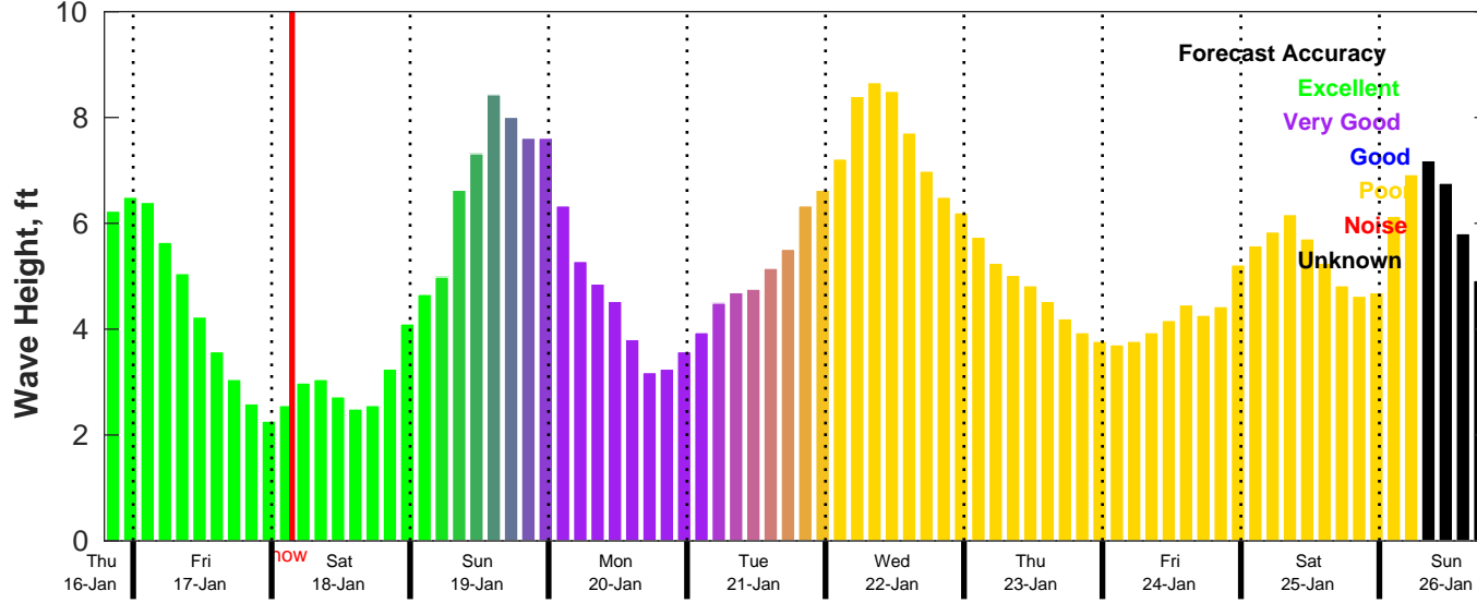
CMEMS Wave Forecast for NDBC 41013 from 16-Jan-2025 19:00:00 to 26-Jan-2025 19:00:00
