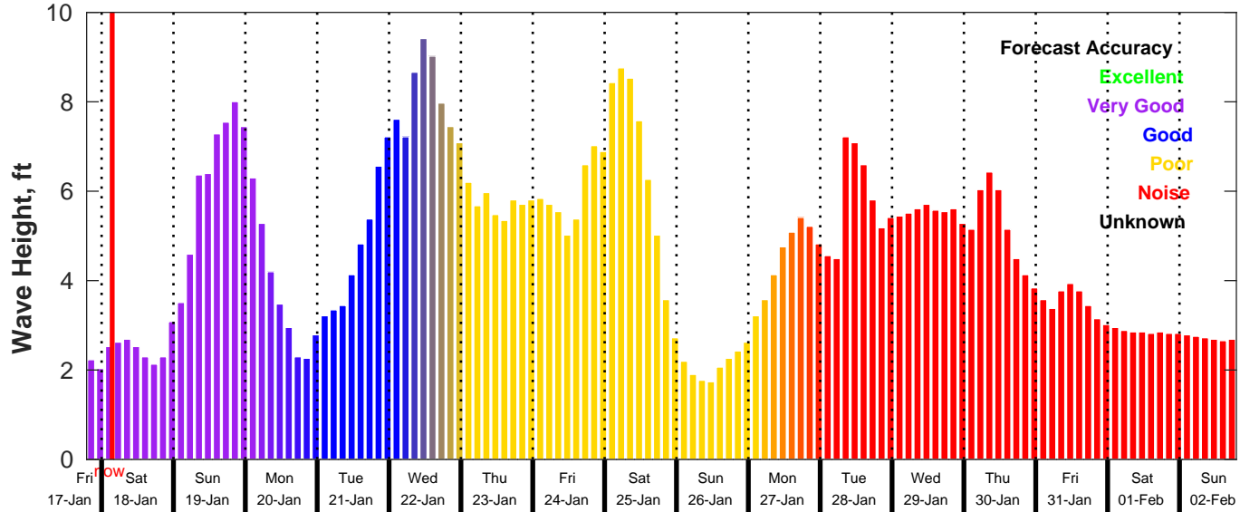
GFS Wave Forecast for NDBC 41013 from 17-Jan-2025 19:00:00 to 02-Feb-2025 19:00:00
