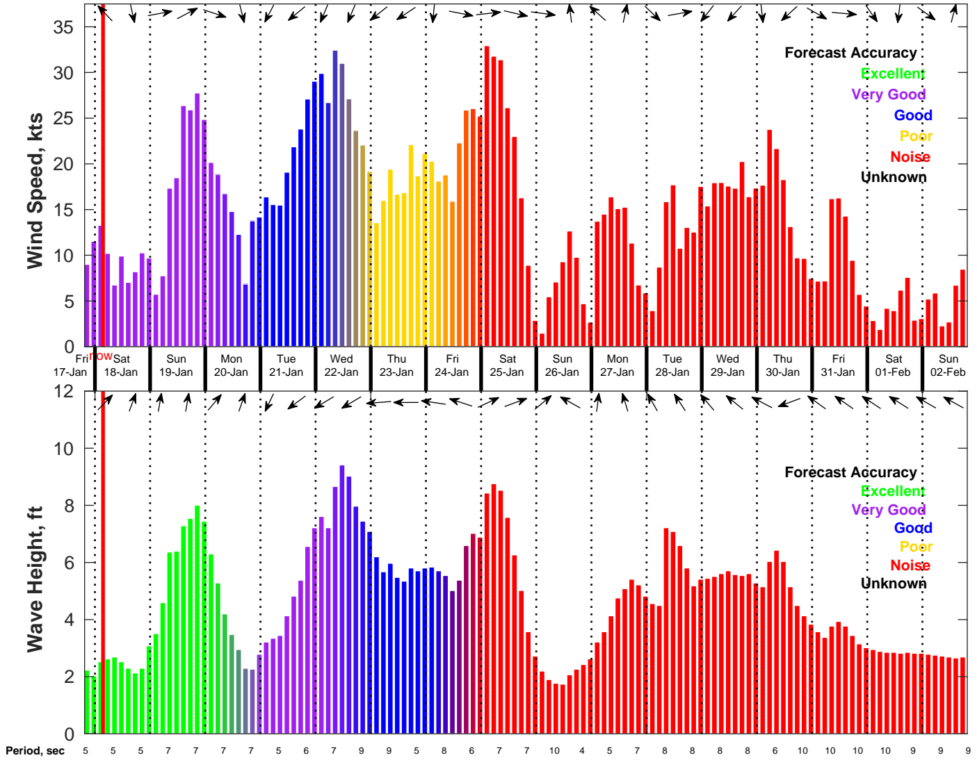
Wind & Wave Forecast for NDBC 41013 from 17-Jan-2025 19:00:00 to 02-Feb-2025 19:00:00
