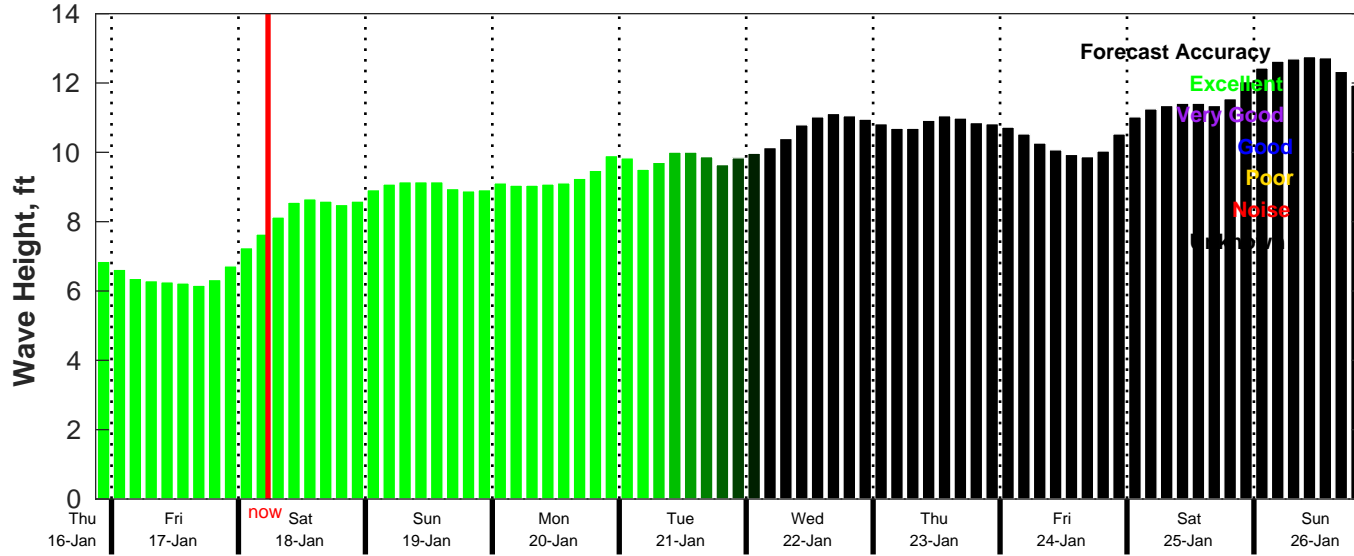
CMEMS Wave Forecast for NDBC 41040 from 16-Jan-2025 21:00:00 to 26-Jan-2025 21:00:00
