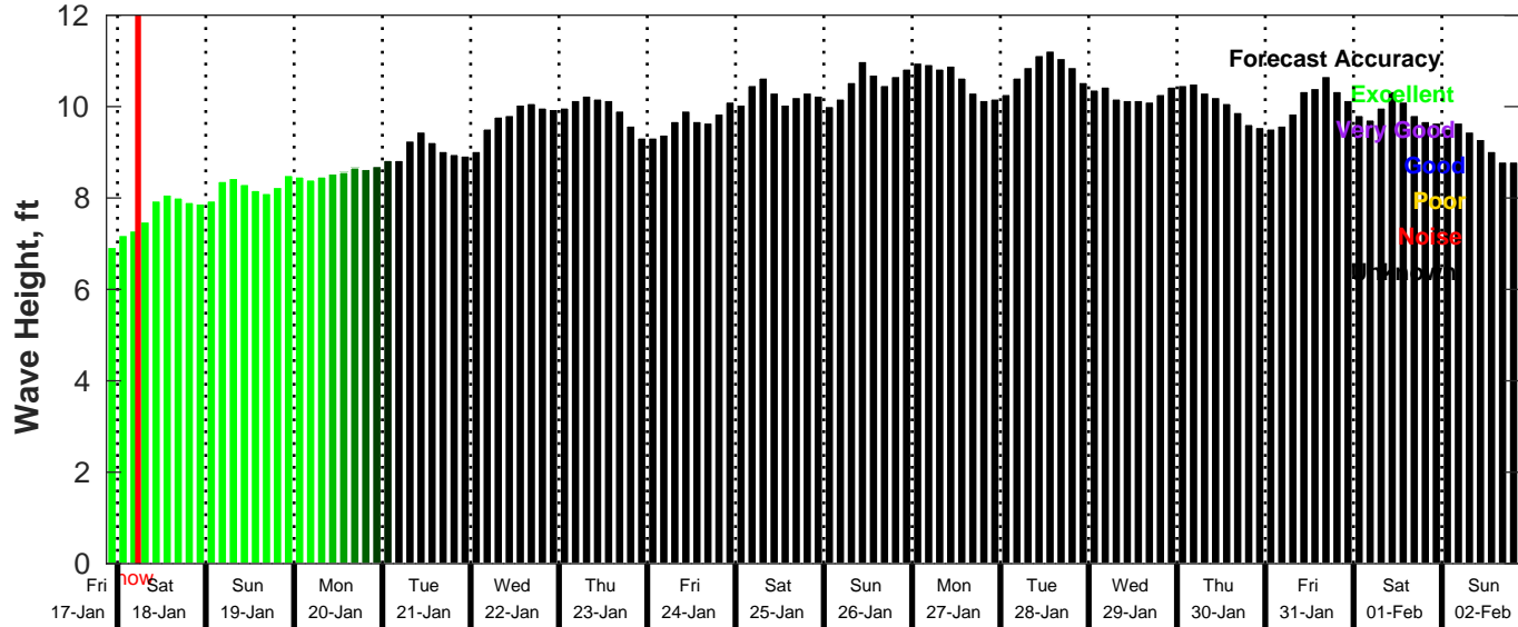
GFS Wave Forecast for NDBC 41040 from 17-Jan-2025 21:00:00 to 02-Feb-2025 21:00:00
