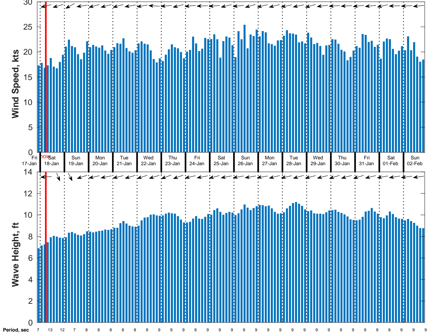
Wind & Wave Forecast for NDBC 41040 from 17-Jan-2025 21:00:00 to 02-Feb-2025 21:00:00
