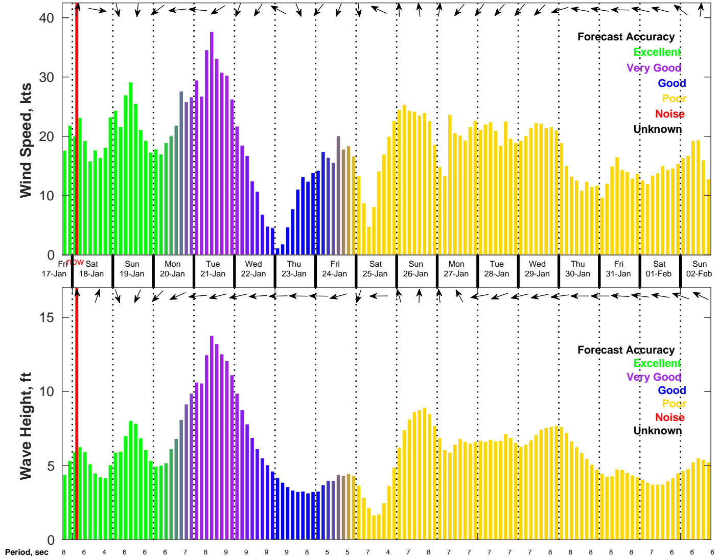
Wind & Wave Forecast for NDBC 42019 from 17-Jan-2025 18:00:00 to 02-Feb-2025 18:00:00
