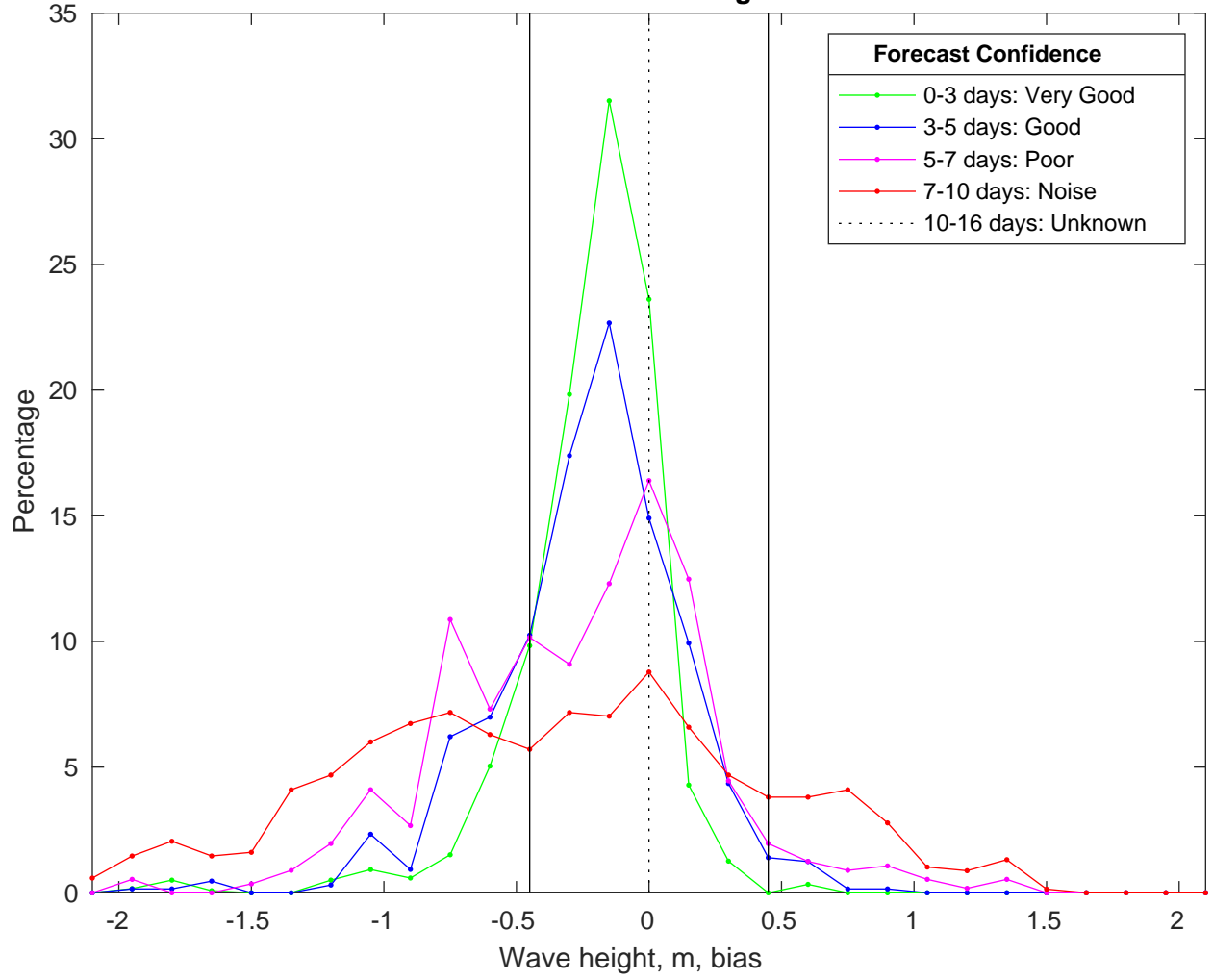
NDBC 42020 vs CMEMSWaves Bias Histogram: 18-Jan-2025
