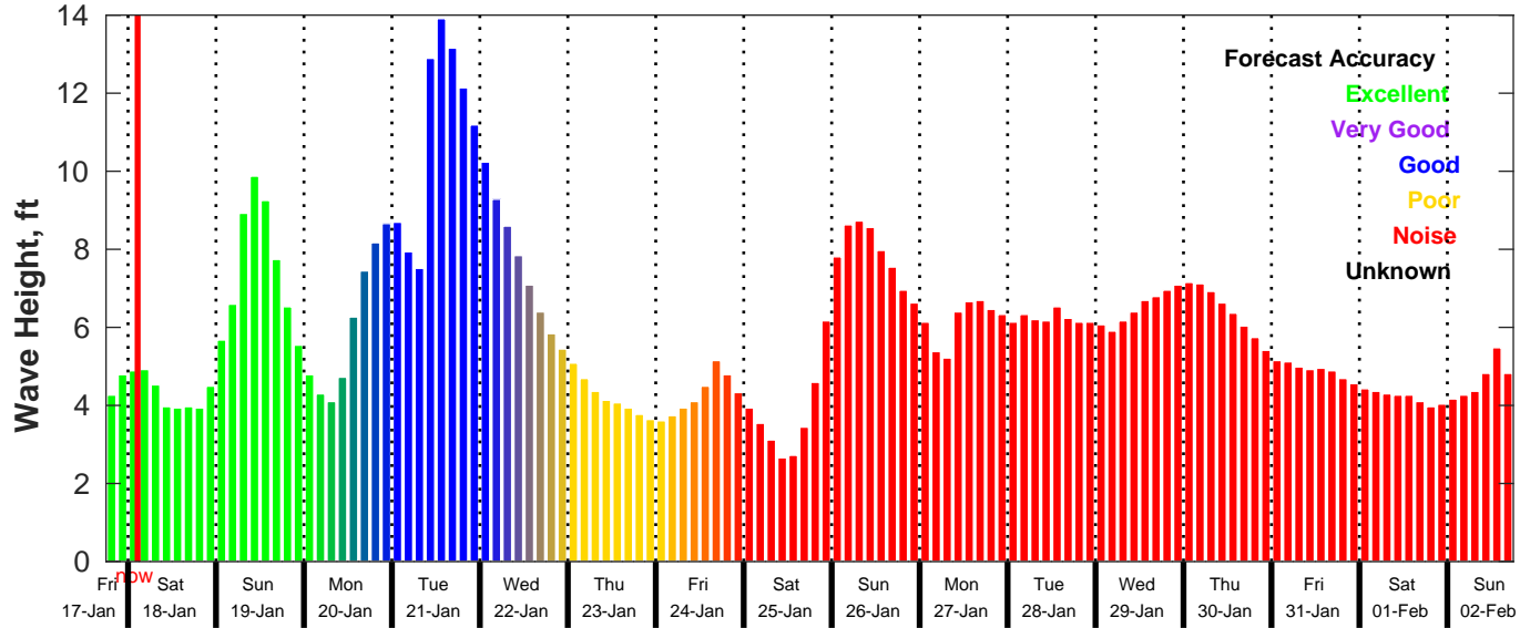
GFS Wave Forecast for NDBC 42020 from 17-Jan-2025 18:00:00 to 02-Feb-2025 18:00:00
