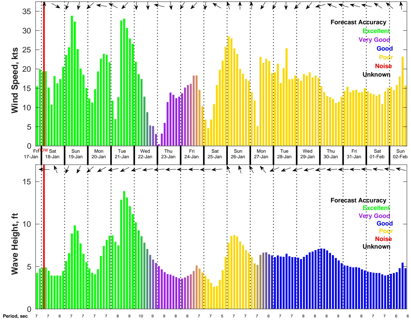
Wind & Wave Forecast for NDBC 42020 from 17-Jan-2025 18:00:00 to 02-Feb-2025 18:00:00
