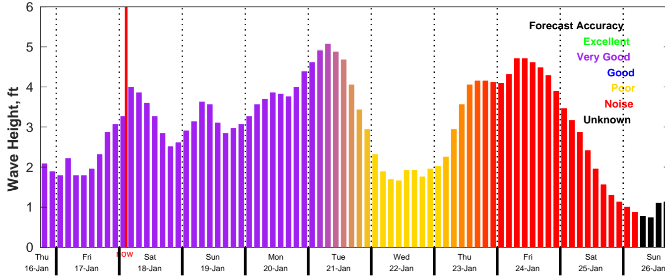
CMEMS Wave Forecast for NDBC 42035 from 16-Jan-2025 18:00:00 to 26-Jan-2025 18:00:00
