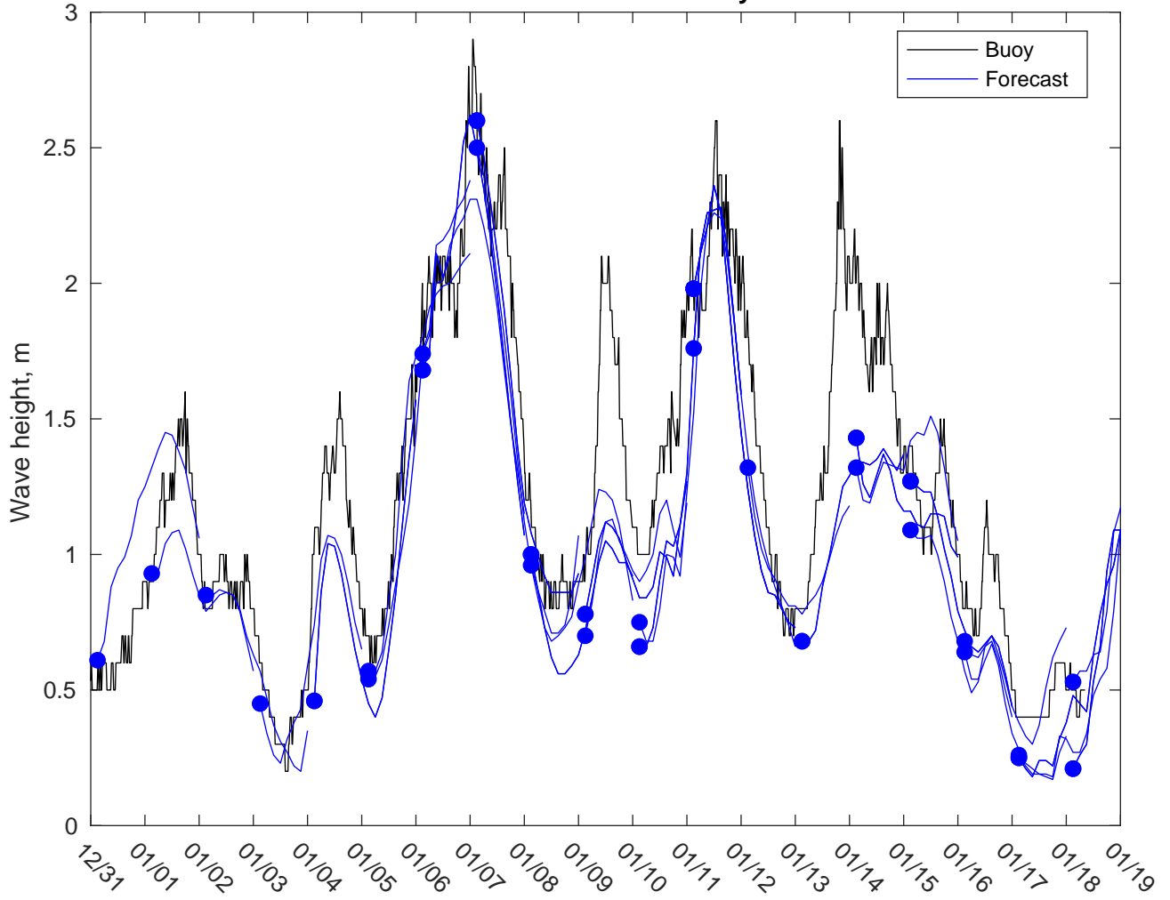
NDBC 42036 vs CMEMSWaves: 3 to 5 day forecast
