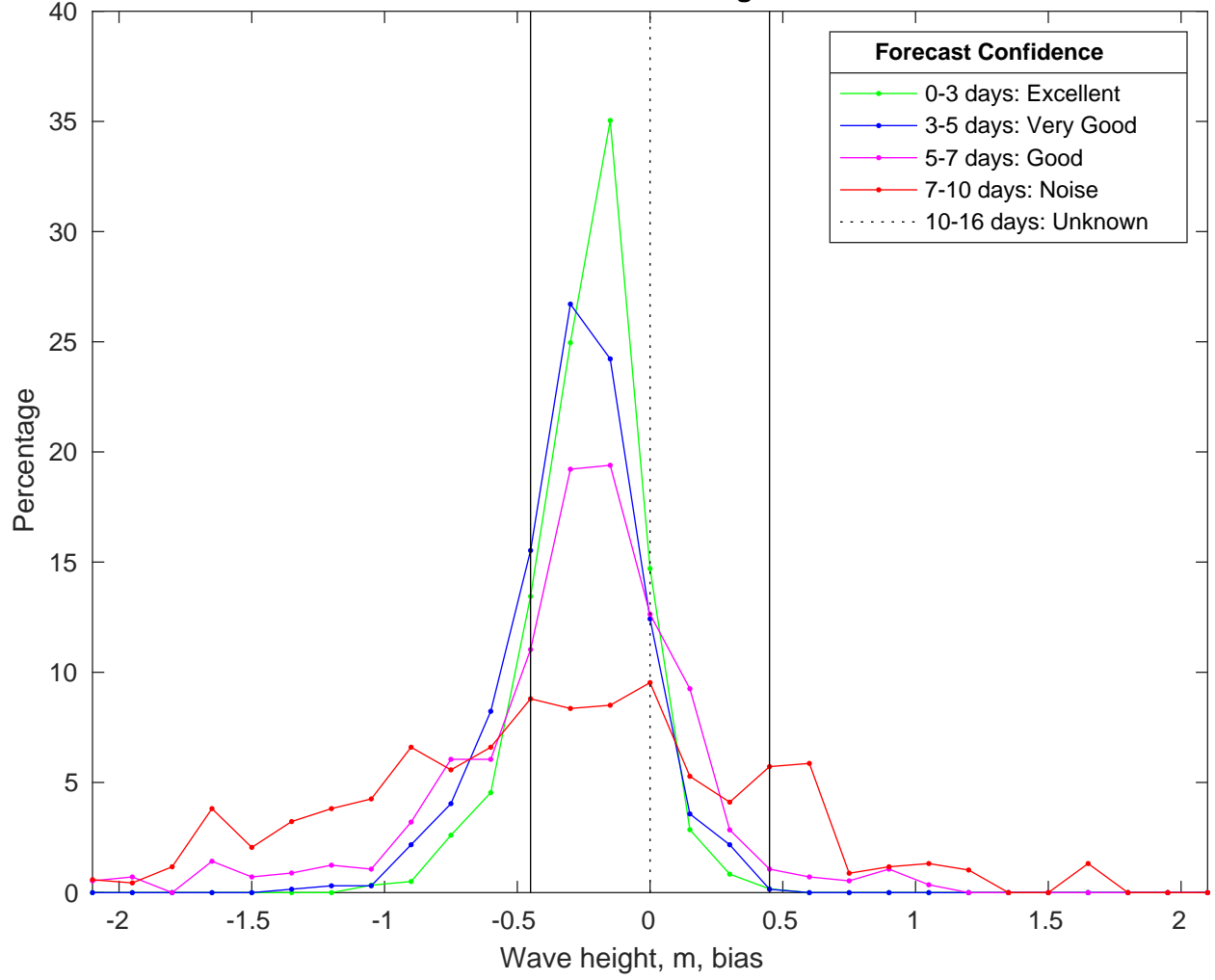
NDBC 42036 vs CMEMSWaves Bias Histogram: 18-Jan-2025
