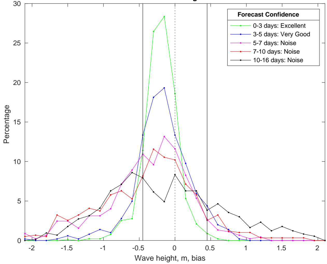
NDBC 42036 vs GFSWaves Bias Histogram: 18-Jan-2025
