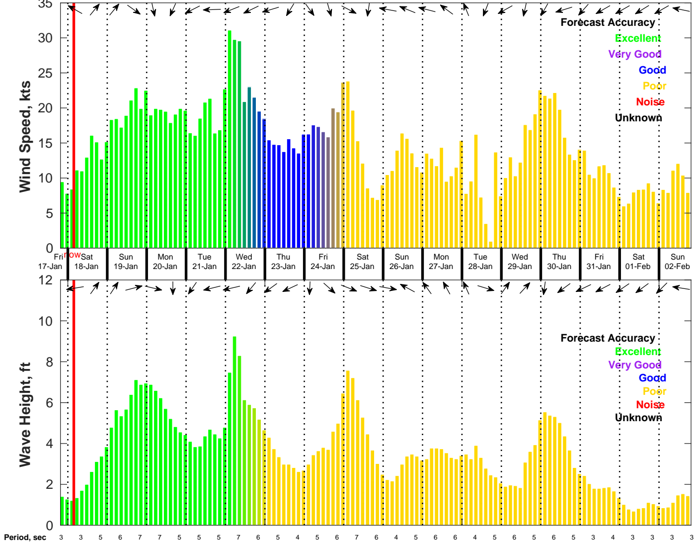
Wind & Wave Forecast for NDBC 42036 from 17-Jan-2025 19:00:00 to 02-Feb-2025 19:00:00
